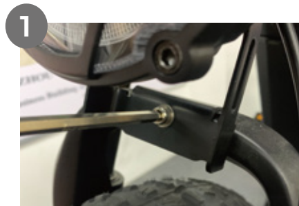
1. Put the headlight on the arch of the fork. Locate the bolt hole.
