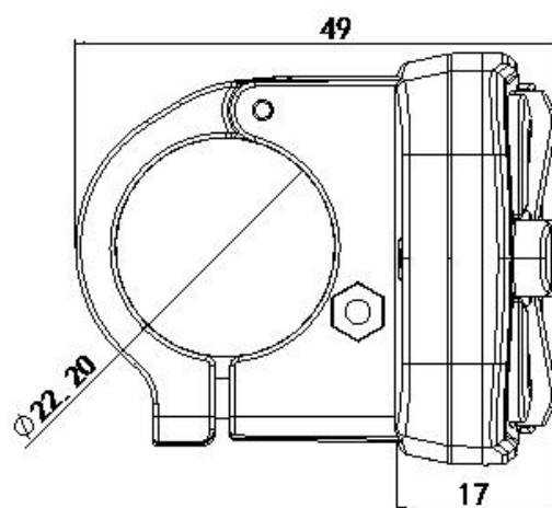
Figure 3-6: F9 Button Side View Dimensions
