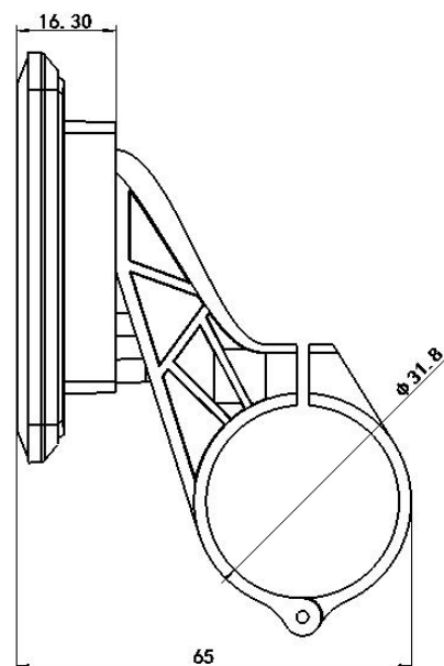
Figure 3-4: DR-208 Instrument Side View Dimensions
